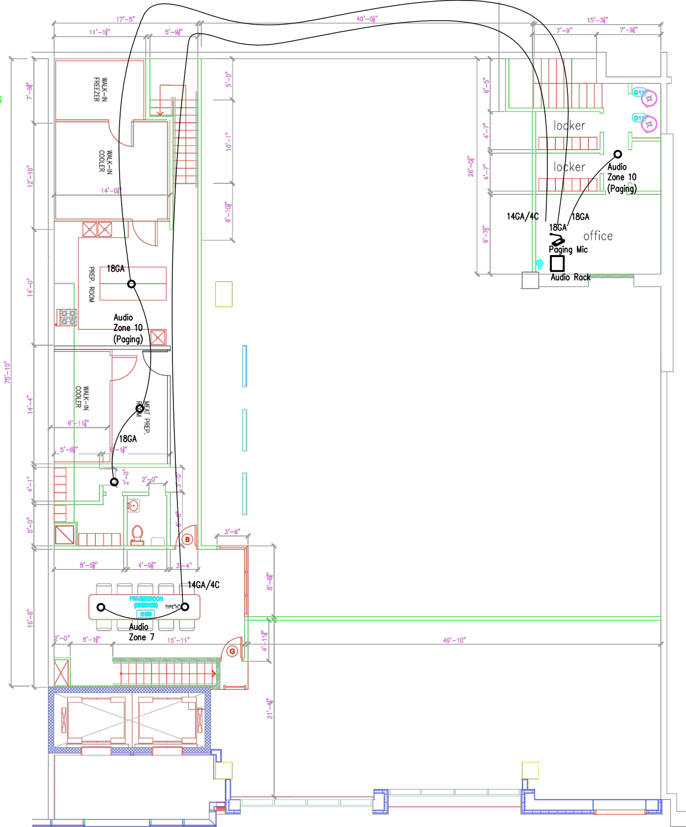
mezzanine
