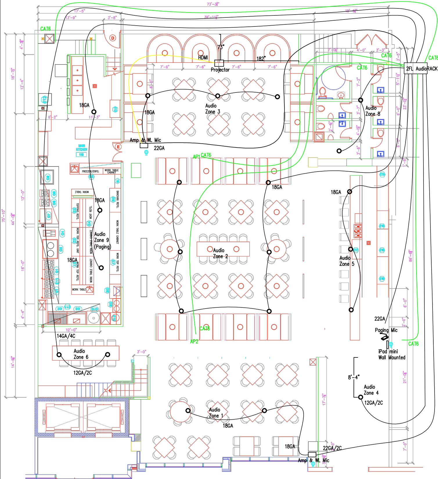
floor plan
